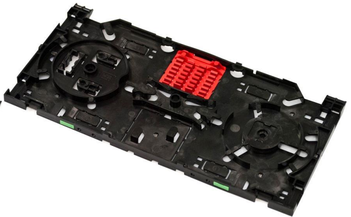
SCM-A-12H Cassette with an option for 12 fusion splices and 2 splitters
